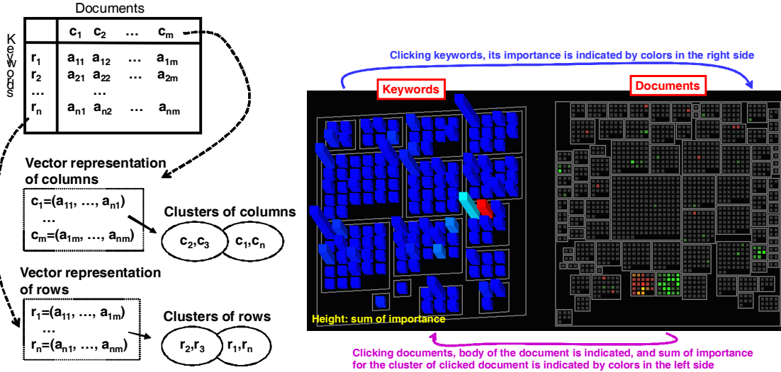
Figure 1. Overview of the newspaper corpus visualization technique applying our own dual hierarchical data visualization technique. (Left) The technique first generates clusters of columns and rows of keyword-document matrix data. (Right) The technique then visualizes the two sets of clusters applying the dual hierarchical data visualization technique.
