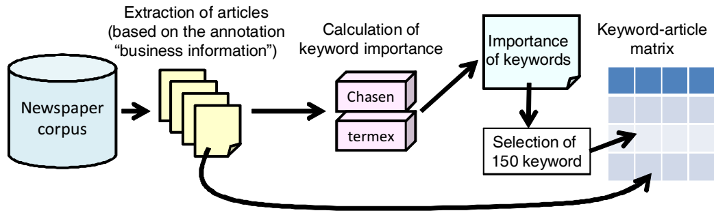
Figure 2. Processing flow for keyword-document matrix construction from Japanese newspaper corpus.
